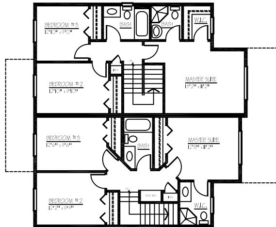
UPPER FLOOR PLAN - 660 SQ. FT. - PER UNIT
