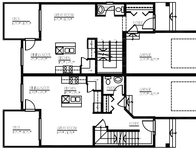
MAIN FLOOR PLAN - 598 SQ. FT. - PER UNIT
