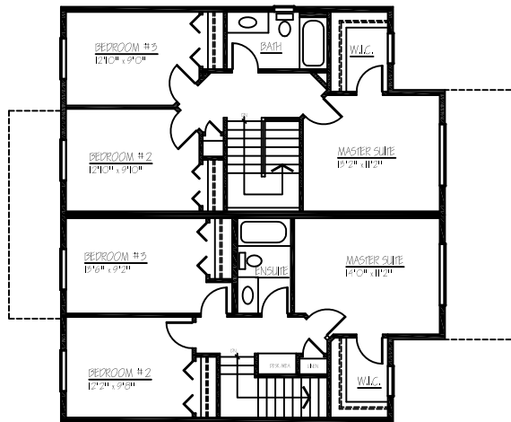
UPPER FLOOR PLAN - 648 SQ. FT. - PER UNIT
