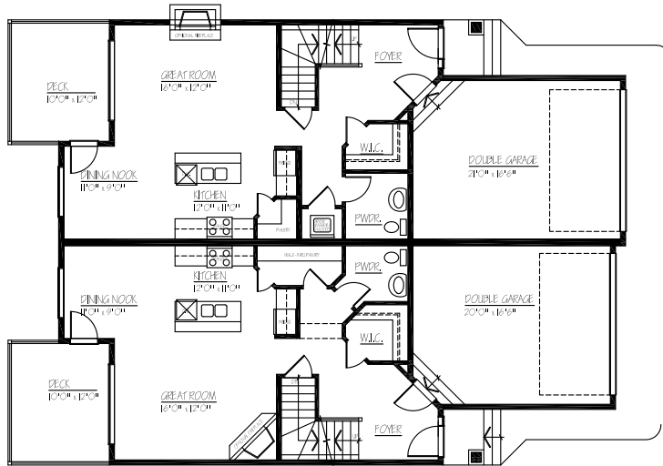
MAIN FLOOR PLAN - 731 SQ. FT.
